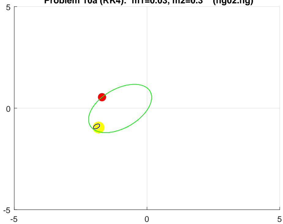
Celestial Mechanics: Two (2) Body Problem Problem 10a (RK4): m_1=0.03 , m_2=0.3 (fig02.fig)
